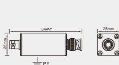
TY-BNC
